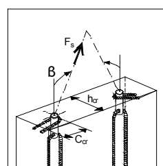
Inclined pull in plane of element
